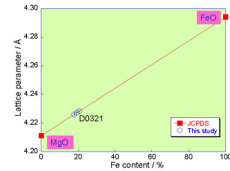
Fig. 4. Lattice parameter of magnesiowüstite as a function of Fe content. From the peak shift of MgO, shown in Fig. 3, we can estimate the Fe content, if it is assumed there is a linear relation between the lattice parameter and Fe content. The Fe content of this run was estimated to be about 20% in molar ratio.
