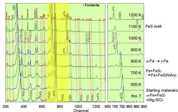
FIG. 5. X-ray diffraction change for the system Fe-FeS 2 -Mg 2 SiO 4 during heating. Mg 2 SiO 4 peaks, marked by stars, remain unshifted more than thermal expansion, even when FeS 2 reacts with Fe, forming FeS (NiAs structure), and Fe transforms to \gamma phase.
