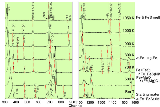
FIG. 2. X-ray diffraction change during heating cycle for the system Fe-FeS 2 -MgO. Pyrite FeS 2 starts reacting with Fe at 700K. At the same time, both MgO and Fe (with bcc structure) peaks drift toward low energy, indicating the expansion of lattice parameters with the same structure. Then \alpha -Fe transforms to \gamma (fcc) phase at 800K. Above 1000K, both Fe and FeS (with NiAs structure) peaks disappeared, meaning these materials melt.
