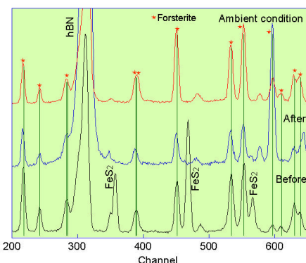
FIG. 6. Comparison of x-ray diffraction patterns at ambient conditions for the system Fe-FeS 2 -Mg 2 SiO 4 . Bottom line shows the diffraction pattern before the experiment. The top two lines collected at different sample positions show the pattern after the experiment. The Mg 2 SiO 4 peaks went back to the original position, while the FeS 2 peaks are lost by the formation of FeS, which is identified as troilite.
