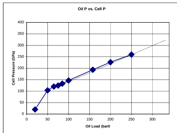
FIG. 3. Pressure vs. oil load.
